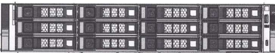
Figure 8. Front View of the R750, 12x 3.5 inches SAS/SATA Chassis
