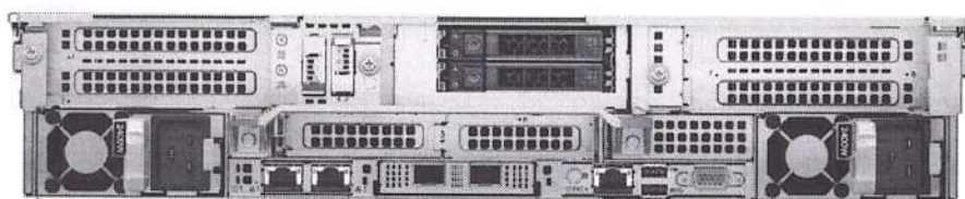
Figure 10. Rear view of the R750 with 2x 2.5 inches storage drives, 6x PCIe Gen4 slots and Hot-plug BOSS
