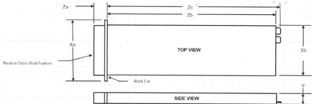
Figure 36. Chassis dimensions
