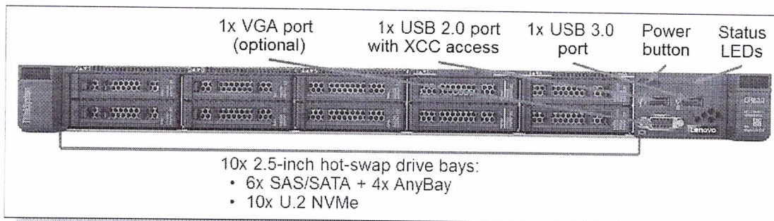
Figure 4. Front view of the SR630: 10x 2.5-inch drive bays
