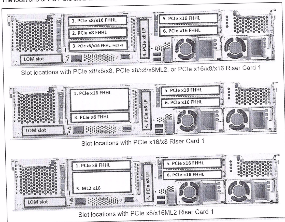
Figure 11. Slot locations
